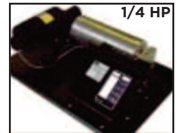
HD443K With 10 inches wide grooved drum Capacity of 30 feet (9.1 m) of cable.
